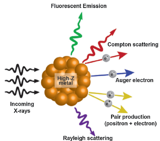
Fig. 1 – Proposed mechanism of metal nanoparticles interaction with radiation. Adapted from Ref. 19
